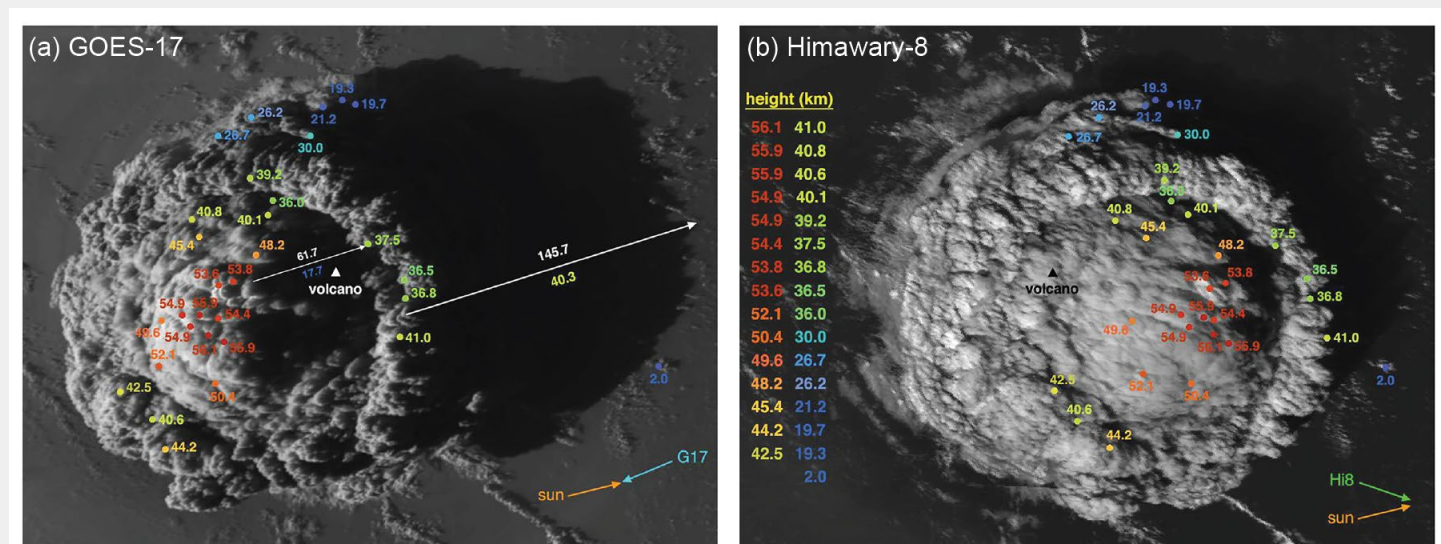
Fig. SB2.3. (From Carr et al. 2022, their caption. Figure used under CC BY 4.0 ): Image of the plume on 15 Jan 2022 at 0430 UTC from (a) GOES-17 and (b) Himawari-8. Colored dots mark manual stereo height estimates (in km), and the white/black triangles show the volcano's location. The white arrows in panel (a) depict the shadow of a plume edge feature and a dome feature, with the shadow length and the derived height given above/below the arrow. Arrows in the lower right of each panel indicate the sun-to-pixel and satellite-to-pixel azimuths.
