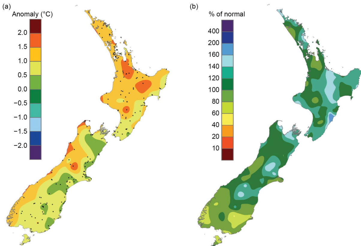
Fig. 7.67. 2022 annual (a) average temperature anomaly ( ^\circ\text{C} ) and (b) total rainfall (% of normal), relative to the 1981–2010 base period. The black dots on (a) represent the locations of climate stations used to create both the temperature and rainfall maps. Note: some data used to create these plots have been identified as not homogenized. As NIWA switches to the 1991–2020 normal period, these data will be homogenized (Source: NIWA.)
