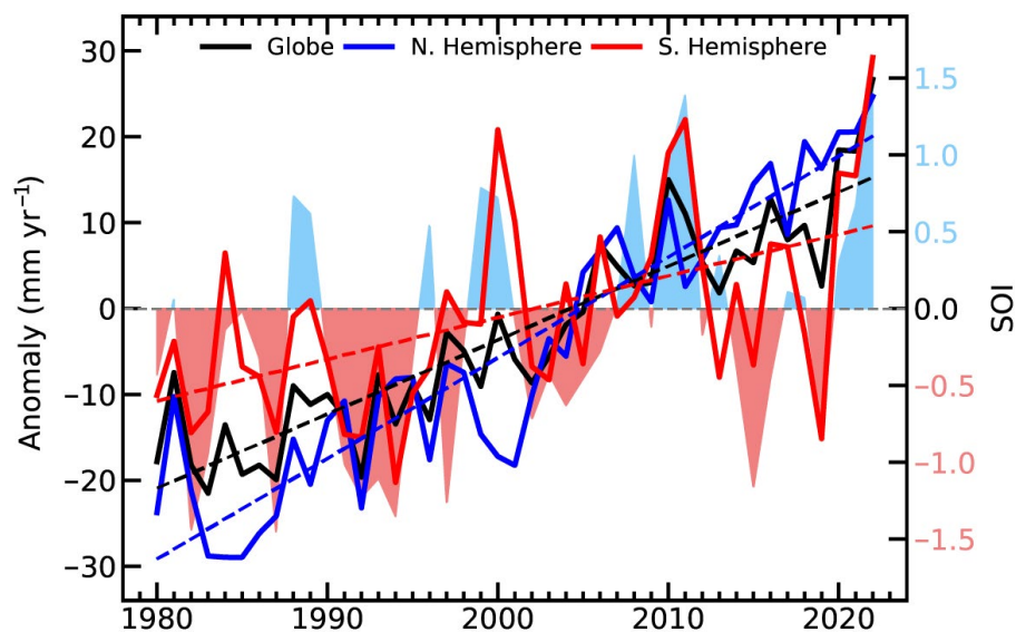
Fig. 2.41. Land evaporation anomalies (mm yr -1 ; 1991–2020 base period) for the Northern Hemisphere, Southern Hemisphere, and the entire globe (blue, red, and black solid lines, respectively). Linear trends in evaporation (dashed lines) and the Southern Oscillation Index (SOI) from CRU (right axis, shaded area) are also shown. (Sources: GLEAM; https://crudata.uea.ac.uk/cru/data/soi/ .)
