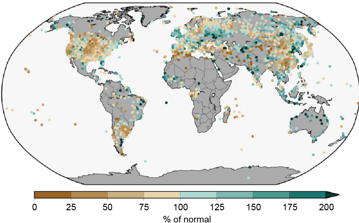
Fig. A4.1. Land-only percent of normal precipitation during (a) JJA 2022 and (b) SON 2022 (relative to a 1961–1990 base period). The figure is provided by NOAA NCEI and the data are from GHCN-M version 4beta (Menne et al. 2018).
